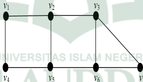
Gambar 2.10 Girth
