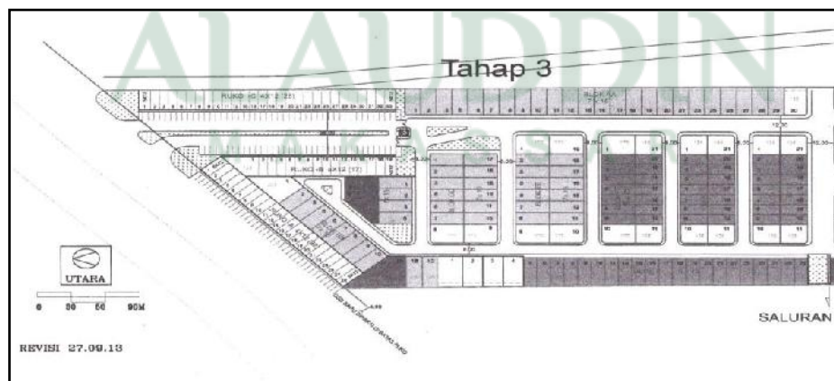
Gambar 4.1. Site plan Perumahan Mutiara Indah Village
