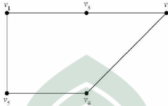
Gambar 2.9 Cycle
