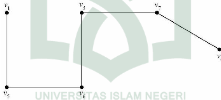
Gambar 2.8 Path
