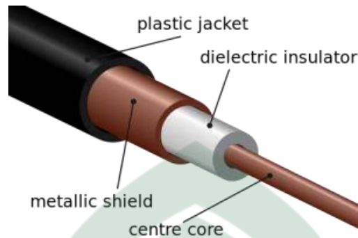
Gambar 2.15 Kabel Coaxial
