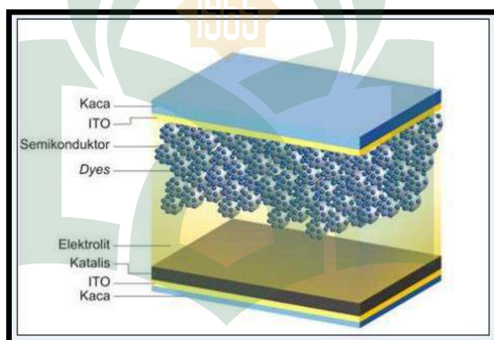
Gambar 2.4. Struktur Dye Sensitized Solar Cell Sumber: http://www.google.co.id
