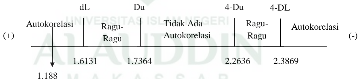
Gambar 4.3 Uji Durbin Watson
