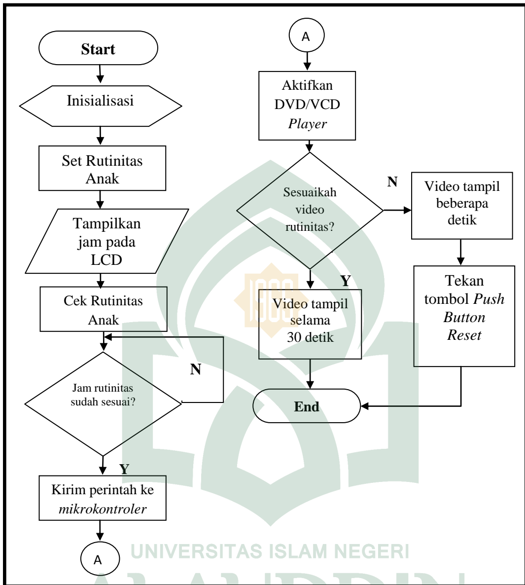
Gambar IV.9 Flowchart Program
