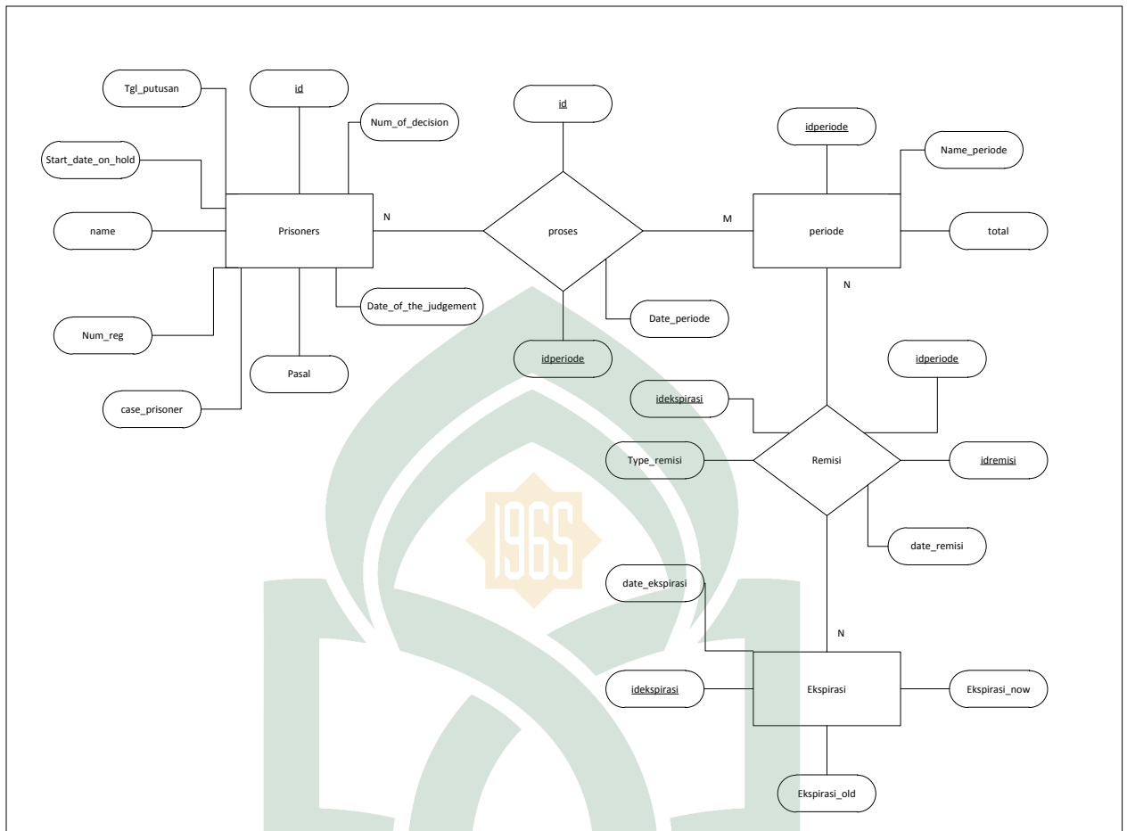
Gambar IV.3. Entity Relationship Diagram (ERD)
