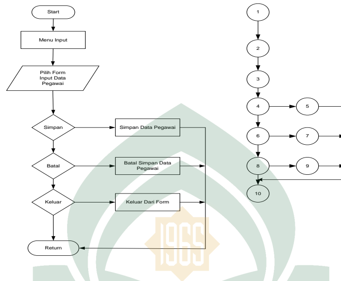
Gambar V. 3 Flowchart dan Flowgraph Form Menu Input Data Pegawai
