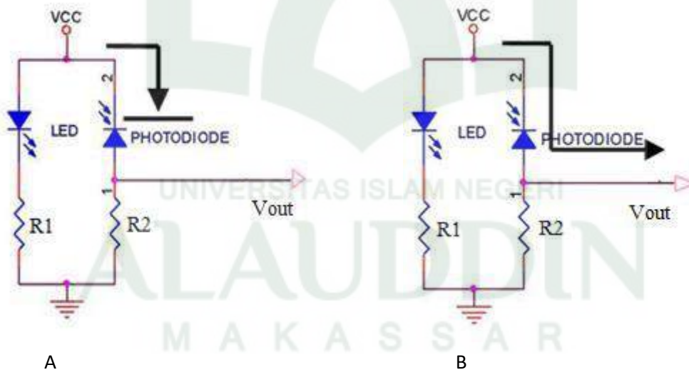
Gambar II.8 Rangkaian prinsip kerja sensor photodiode
