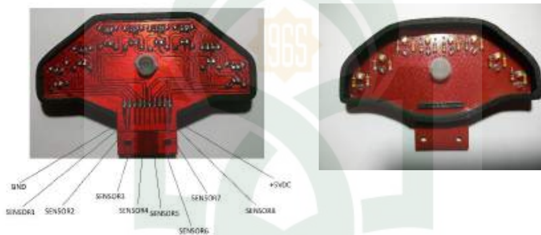
Gambar V.4 Sensor Photodioda
