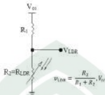
Gambar II.2 Rangkaian LDR
