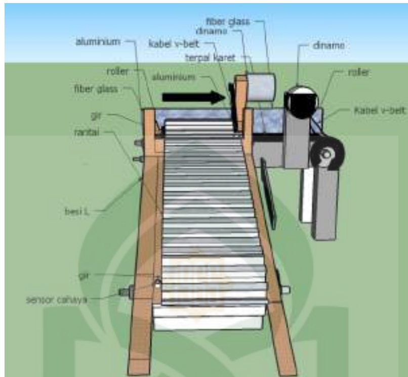
Gambar III.1 Tampak depan
