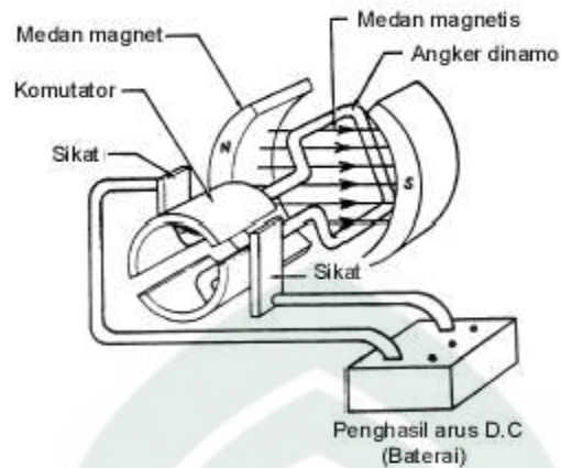
Gambar II.3 Motor DC Sederhana
