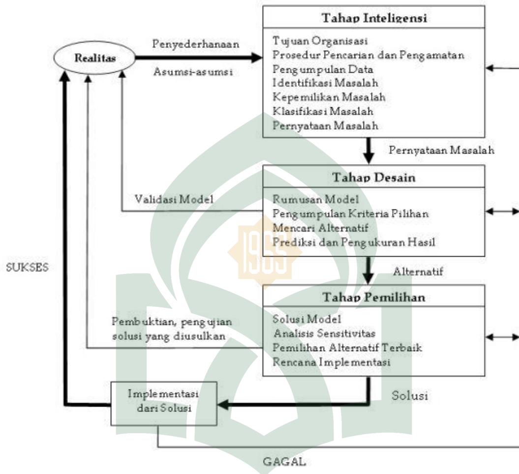
Gambar II.2 Proses Pengambilan Keputusan (Turban, 2005)
