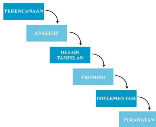
Gambar 2.1 Waterfall Model
