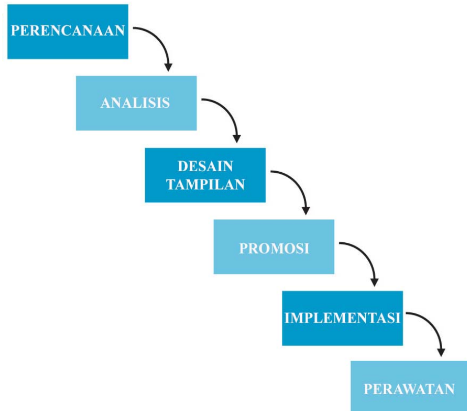
Gambar 4.11 Waterfall Model
