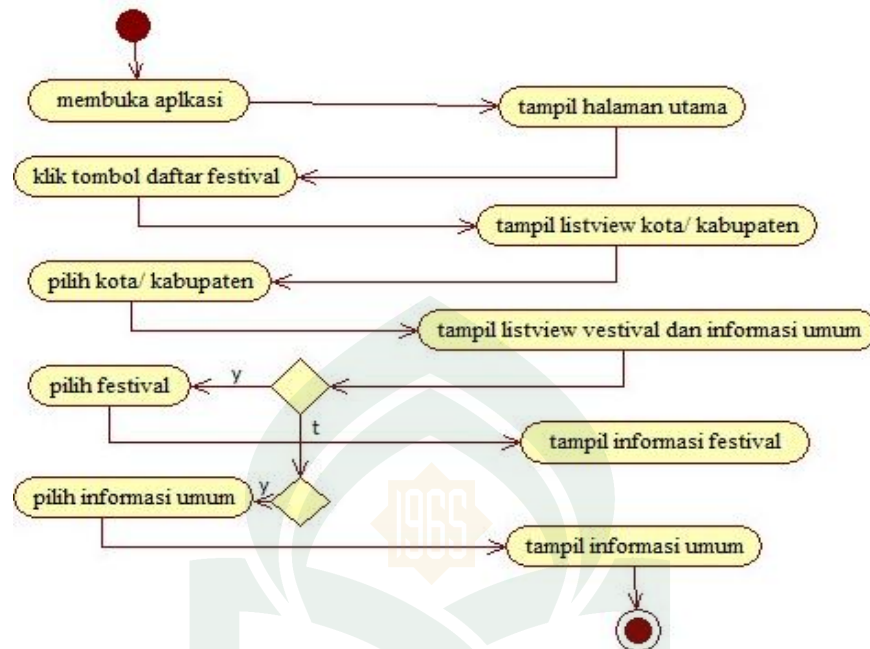
Gambar IV. 12. Activity Diagram Daftar Festival
