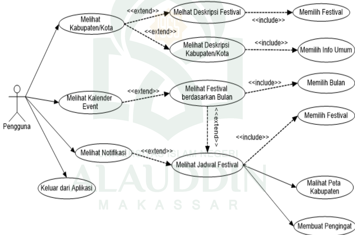
Gambar IV. 6. Use case diagram
