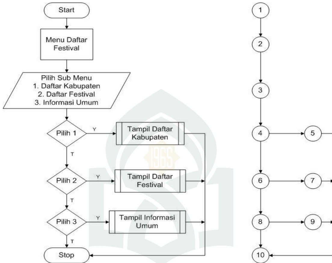
Gambar V. 23. Flowchart dan Flowgraph Daftar Festival
