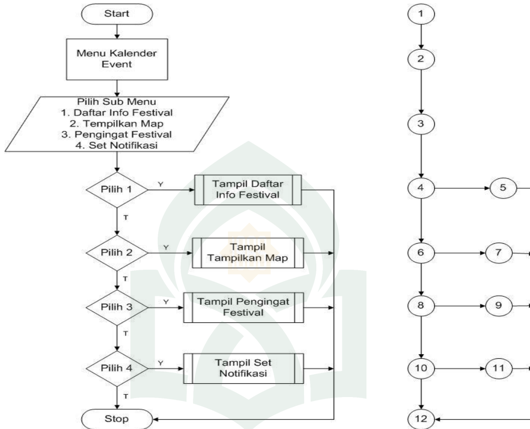
Gambar V. 24. Flowchart dan Flowgraph Kalender Event
