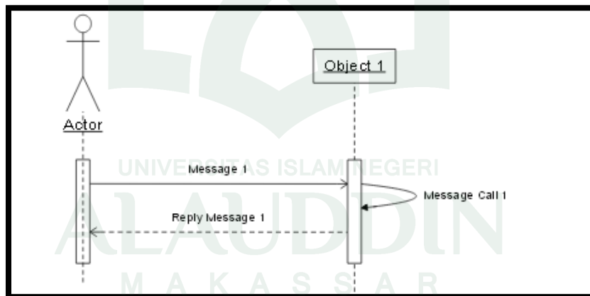
Gambar II. 5. Model Sequece Diagram (Munawar, 2005)
