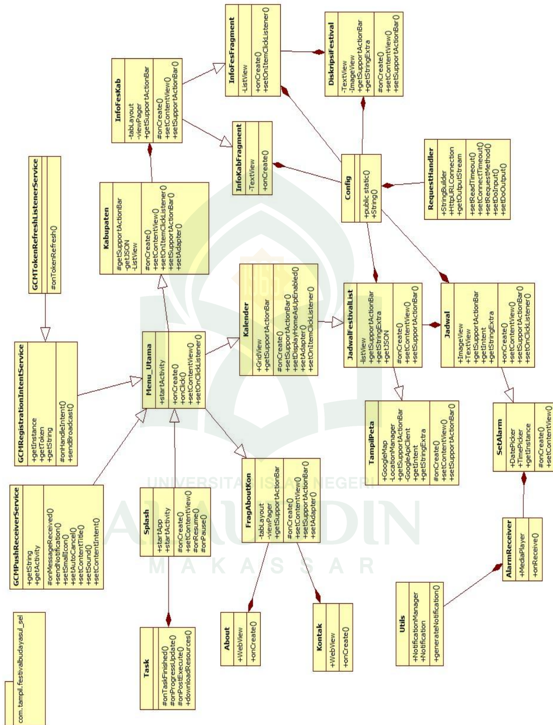
Gambar IV. 15. Class diagram
