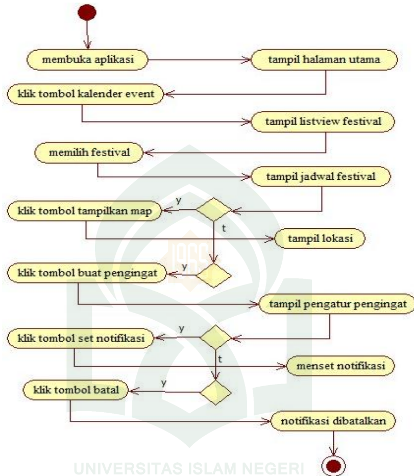
Gambar IV. 14. Activity Diagram Kalender Event
