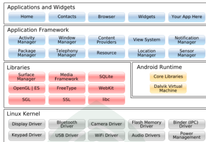
Gambar II.1. Arsitektur Android (Arifin, 2015)
