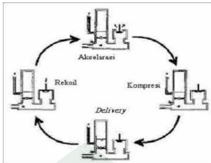
Gambar 2.9 Prinsip kerja pompa hydram
