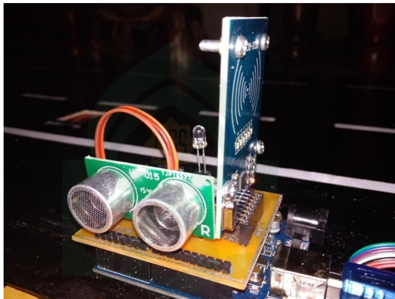
Gambar V. 5 Pengujian Sensor Ping
