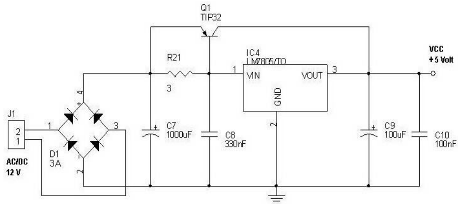
Gambar IV. 5 Rangkaian Power Supply
