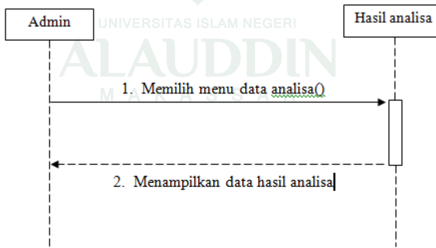
Gambar IV.8 Sequence Diagram hasil analisa
