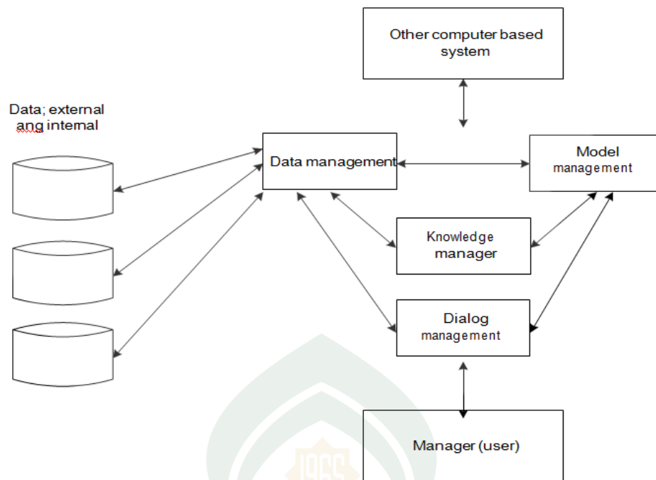
Gambar II. 1. Model Konseptual SPK.
