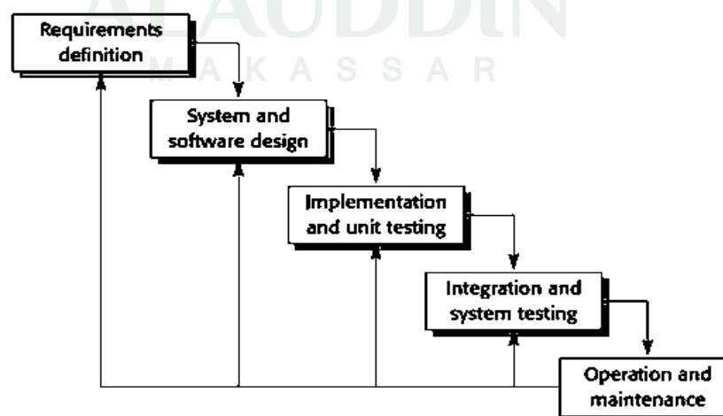
Gambar III. 1. Model Waterfall
