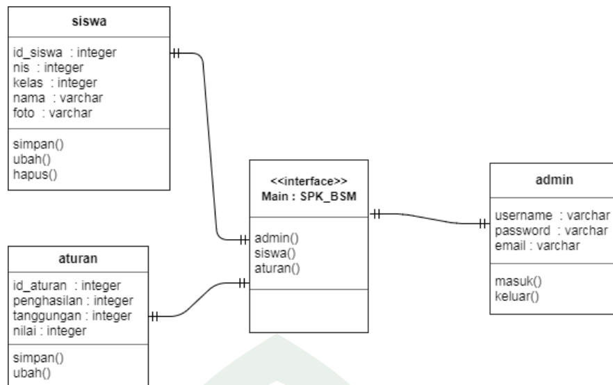
Gambar IV.4 Class Diagram
