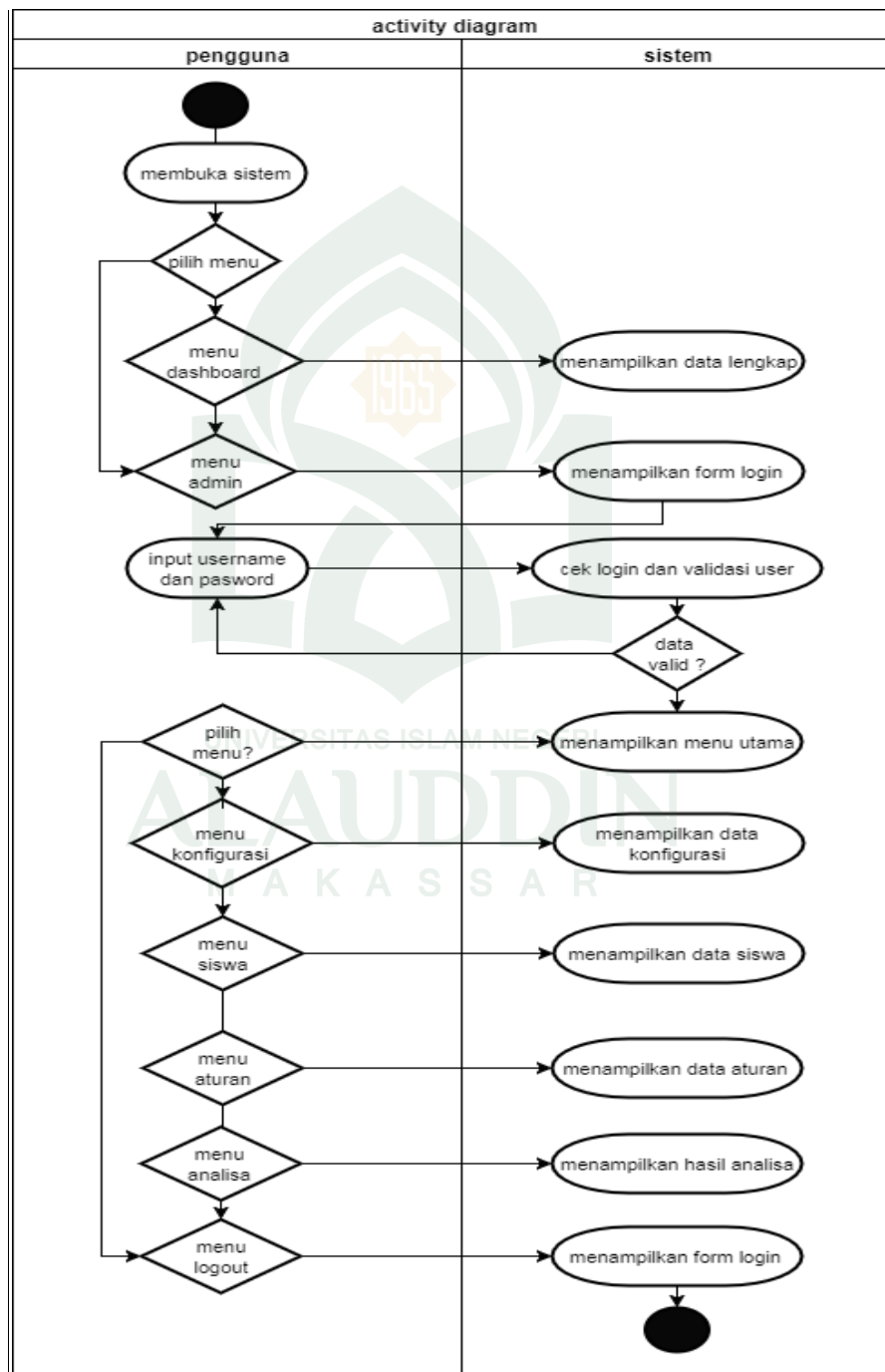
Gambar IV.9 Activity Diagram
