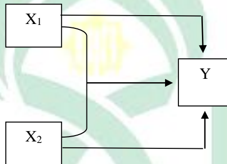
Gambar 3.1 Paradigma Ganda 70
