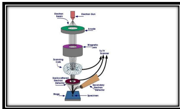
Gambar 2.7 Instrumen Scanning Electron Microscopi- Energi Dispersive X-Ray (SEM/EDX) (Sumber: www.google.com )
