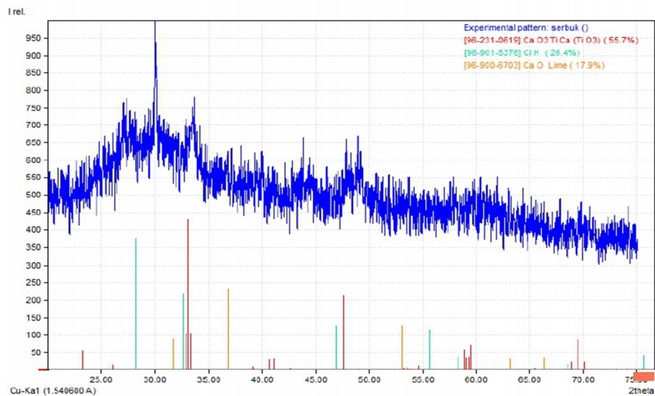
Gambar 4.7 Analisis XRD Hasil Sintesis \text{CaTiO}_3 suhu kalsinasi 1100^\circ\text{C}
