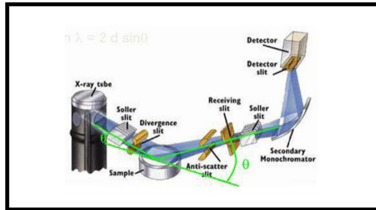
Gambar 2.6: Komponen-konponen X-Ray Diffarction (XRD)
