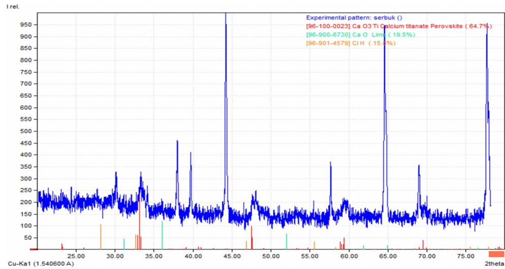
Gambar 4.6 Analisis XRD Hasil Sintesis \text{CaTiO}_3 suhu kalsinasi 1000^\circ\text{C}
