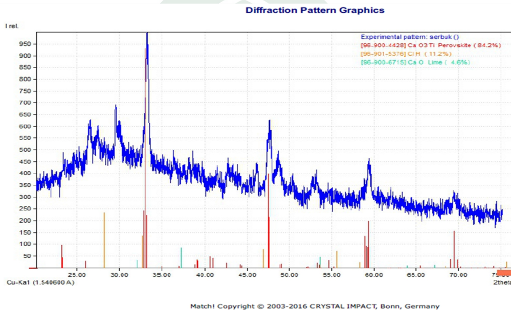
Gambar 4.5 Analisis XRD Hasil Sintesis \text{CaTiO}_3 suhu kalsinasi 900 °C
