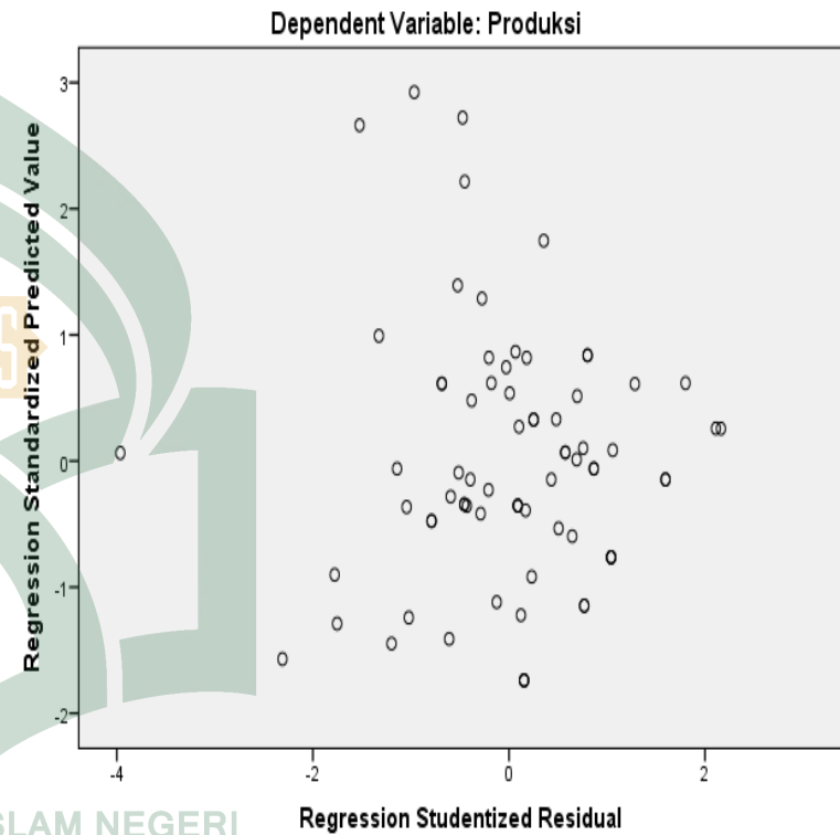
Scatterplot
