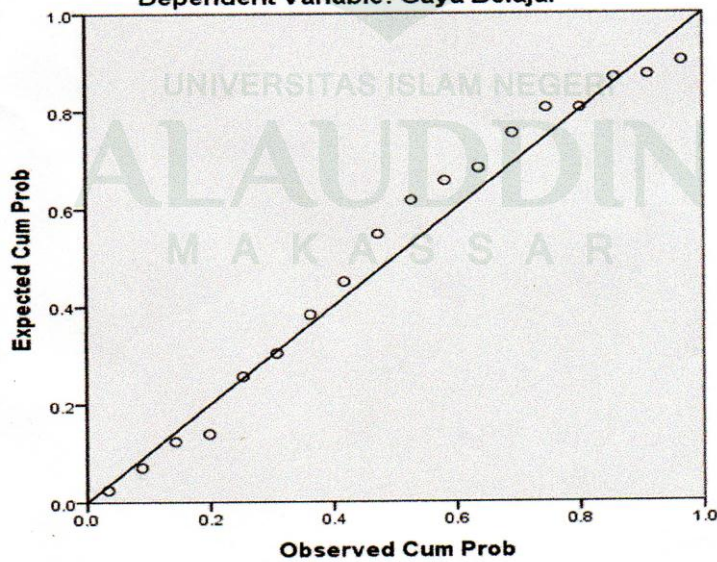
Normal P-P Plot of Regression Standardized Residual Dependent Variable: Gaya Belajar
