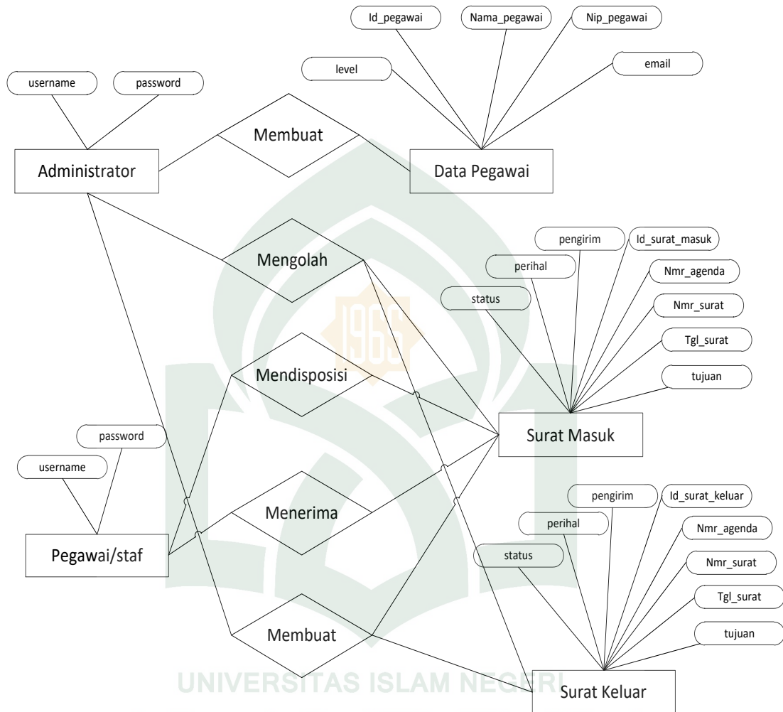
Gambar IV.7 Entity Relationship Diagram
