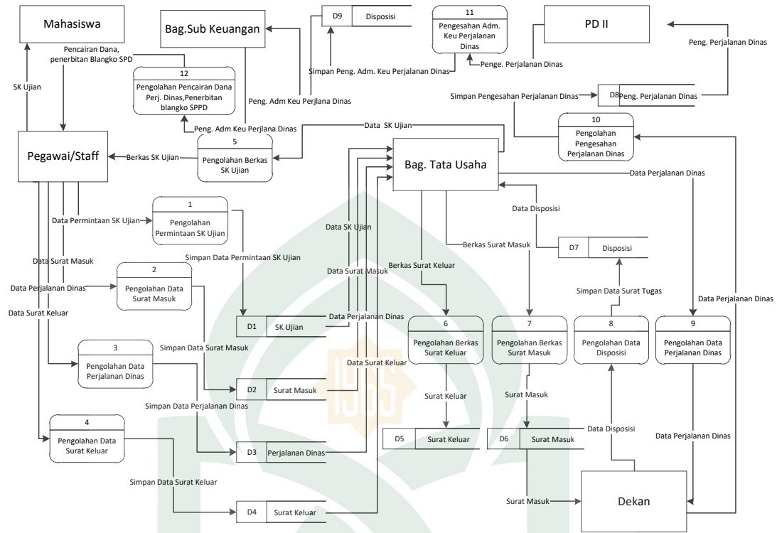
Gambar IV. 6 DFD Level 1 E-Office
