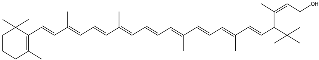
Gambar 2.7 \alpha -cryptoxanthin
