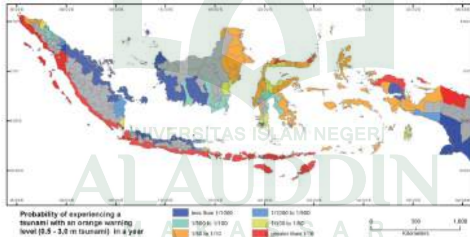
Figure 2-13. Tsunami occurrence probability between 0.5 – 3.0 metres yearly (Source: Horspool., et al. 2013)
