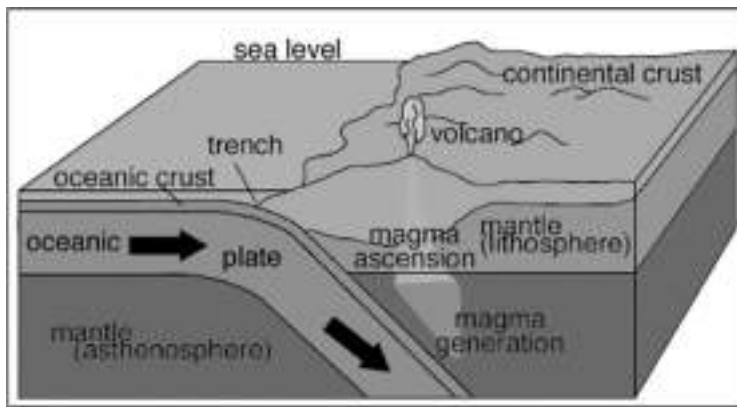
Figure 2-12. Subduction process as configured from platetectonics (Source: platetectonics 2008)
