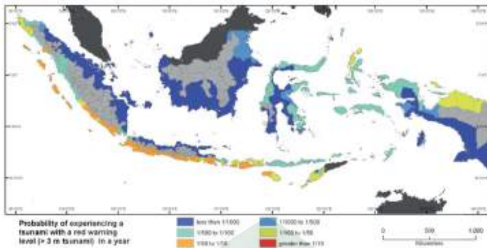
Figure 2-14. Tsunami occurrence probability over 3.0 meters yearly (Source: Horspol., et al.2013)
