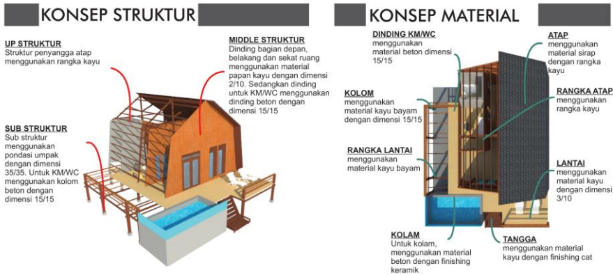
Fig. 5: (left) The concept of structure planning, (right) Material concept
