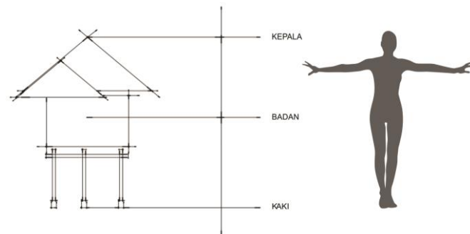
Fig. 3: Form Analogy
