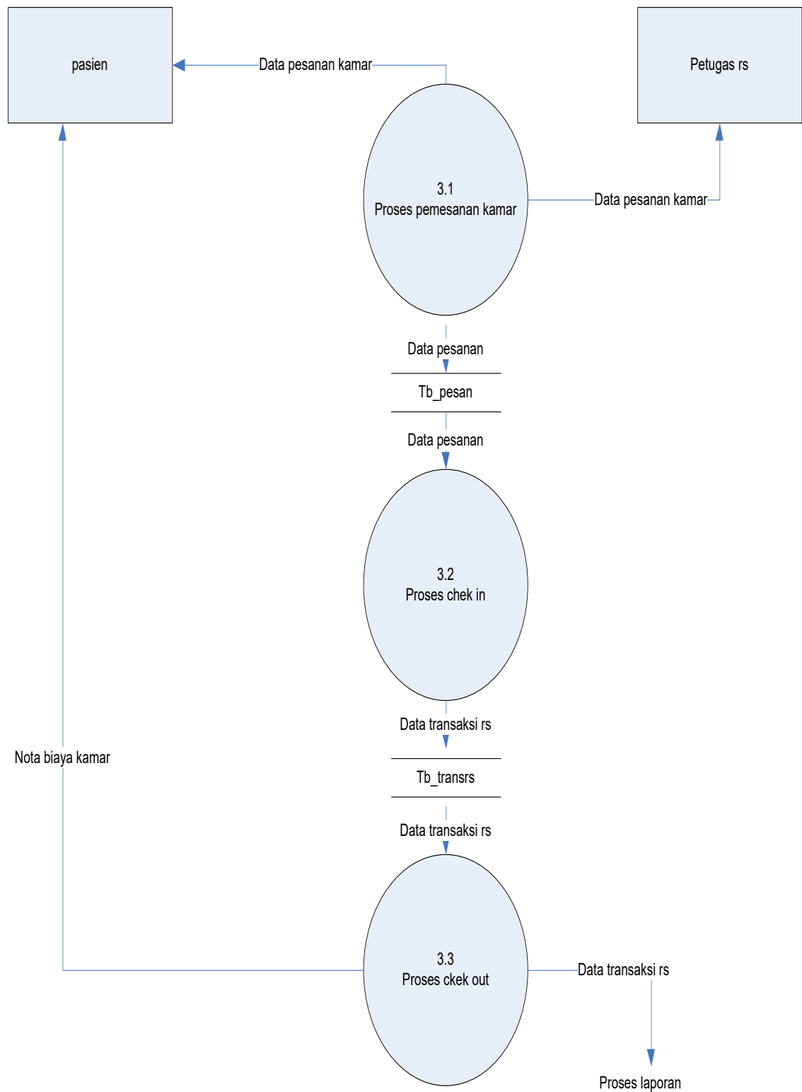
Gambar IV. 6 Diagram level 2 proses 3
