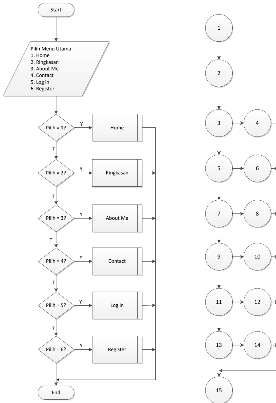
Gambar V.23 Flowchart dan Flowgraph index
