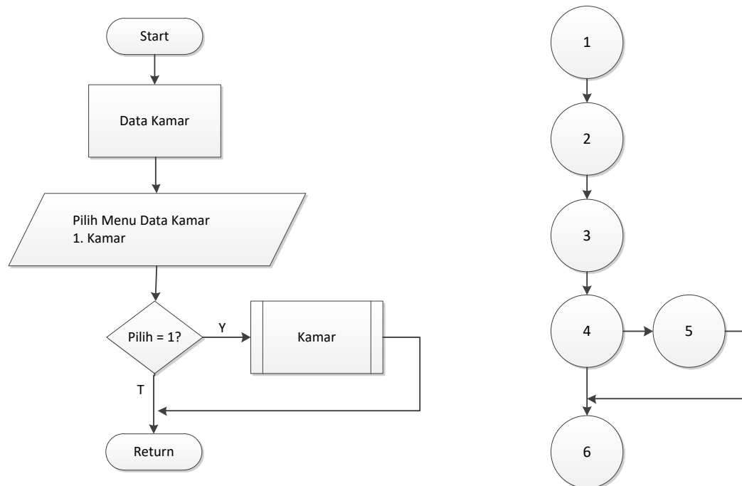
Gambar V.32 Flowchart dan Flowgraph Menu Data Kamar
