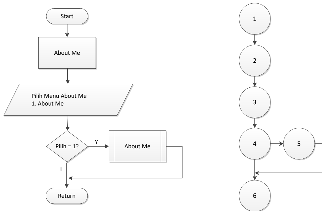
Gambar V.25 Flowchart dan Flowgraph Menu Menu About Me
