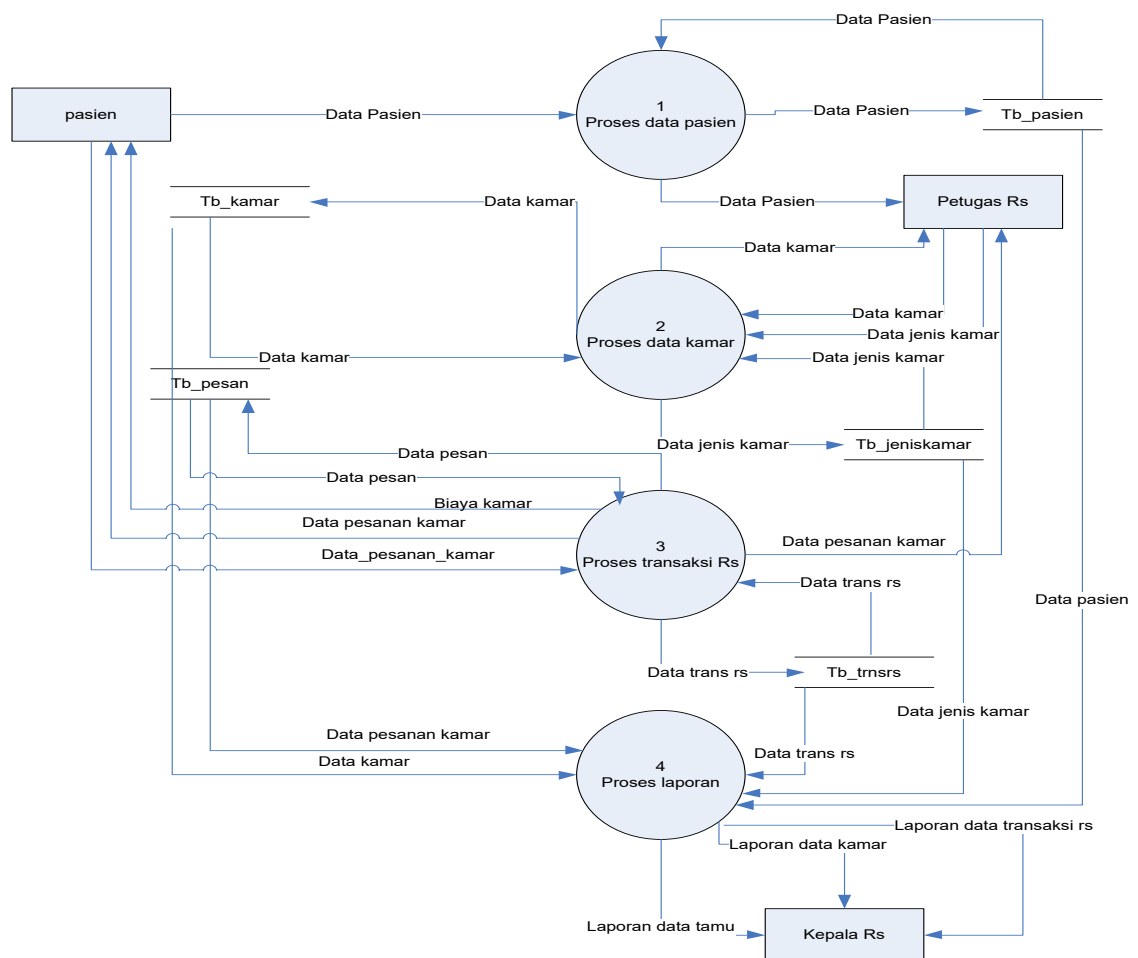
Gambar IV. 5 Diagram Flow Diagram Level 1
