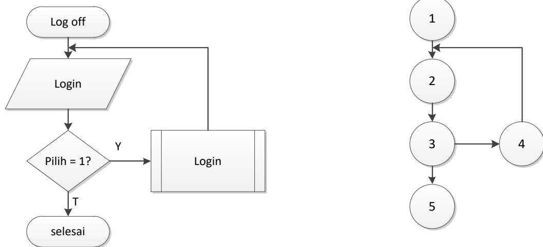
Gambar V.27 Flowchart dan Flowgraph Menu Log in
