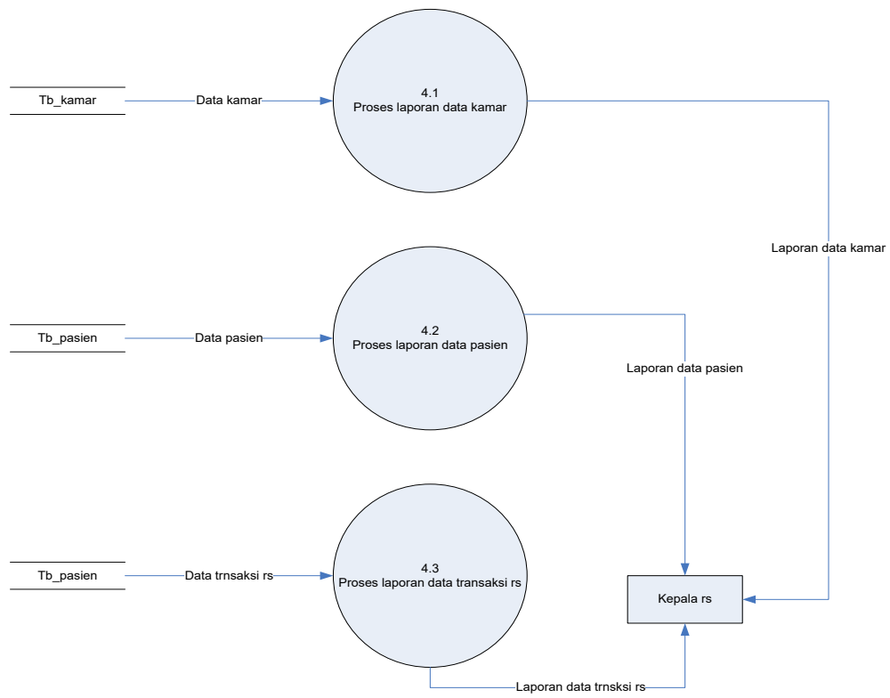
Gambar IV. 7 Diagram level 1 proses 5
