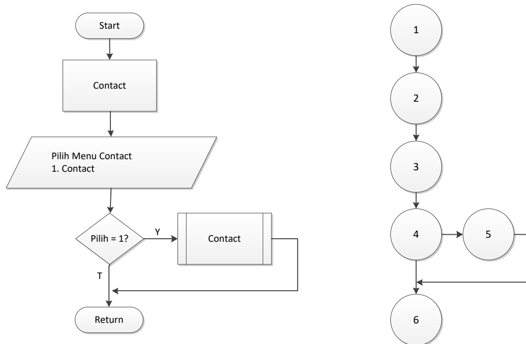
Gambar V.26 Flowchart dan Flowgraph Menu Menu Contact
