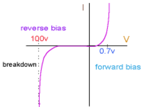
Gambar II.13 Grafik arus dioda
