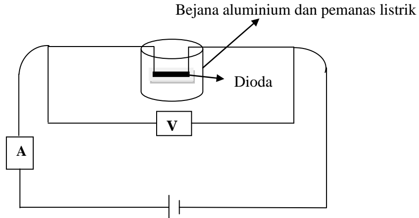
Gambar III.1 Rangkaian alat ukur
