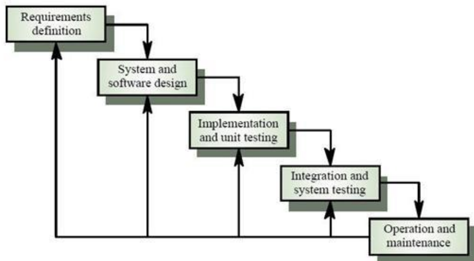
Gambar III.1 Model Waterfall (Pressman, 2001)
