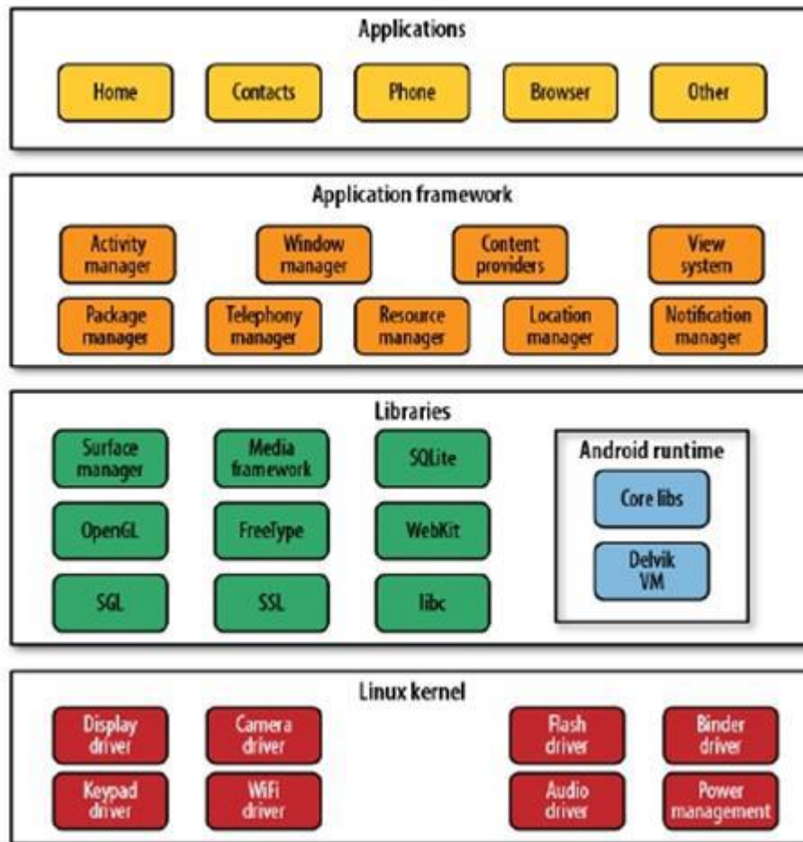
Gambar II.1 Platform Android (Gargenta, 2011)
