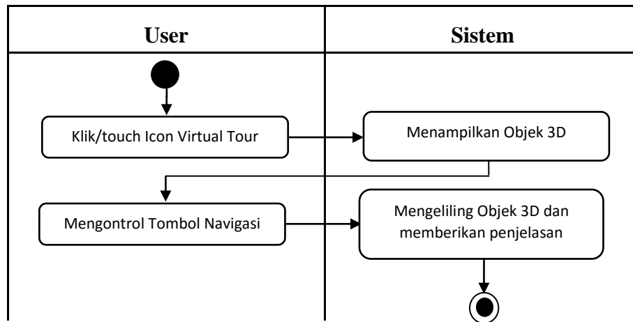
Gambar VI.7 Activity Diagram Menu Virtual Tour
