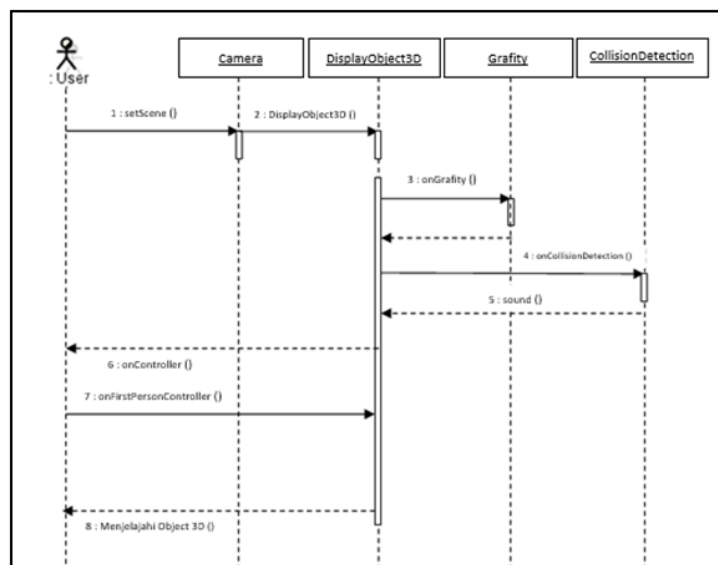
Gambar VI.5 Sequence Diagram Menu Virtual Tour
