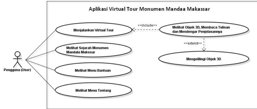
Gambar VI.2 Use Case Diagram
