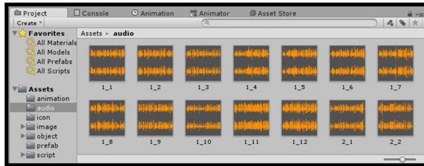
Gambar V.5 File Sound
