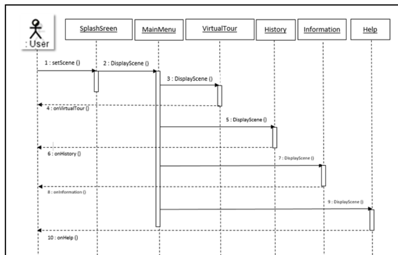
Gambar VI.4 Sequence Diagram Menu
