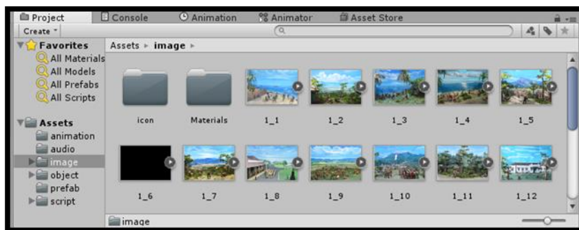
Gambar V.4 File Image
