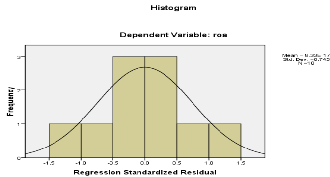
Gambar 4.1. Histogram & Regression Standardized Residual
