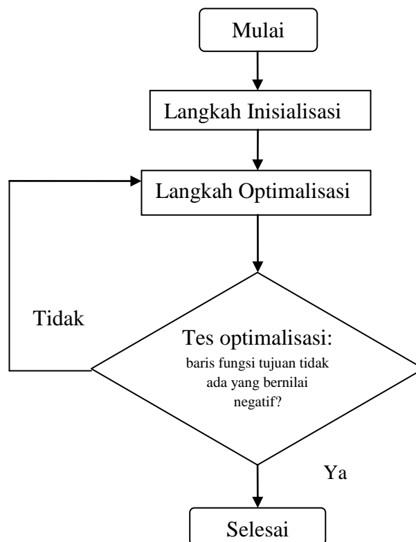
Gambar 2.1 Prosedur Simpleks
