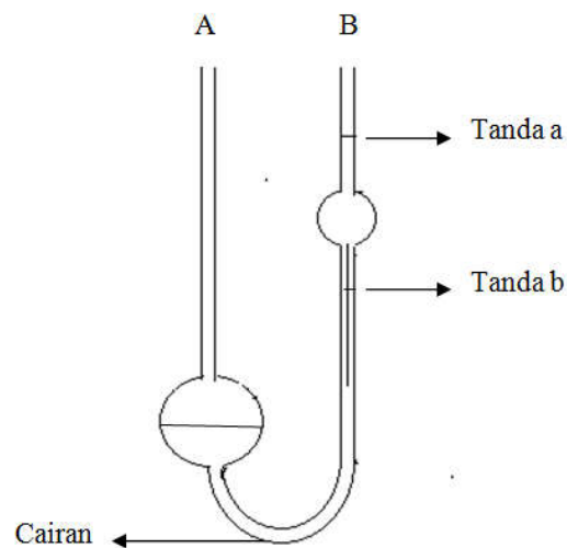
Gambar 2.2: Viskometer Ostwald
